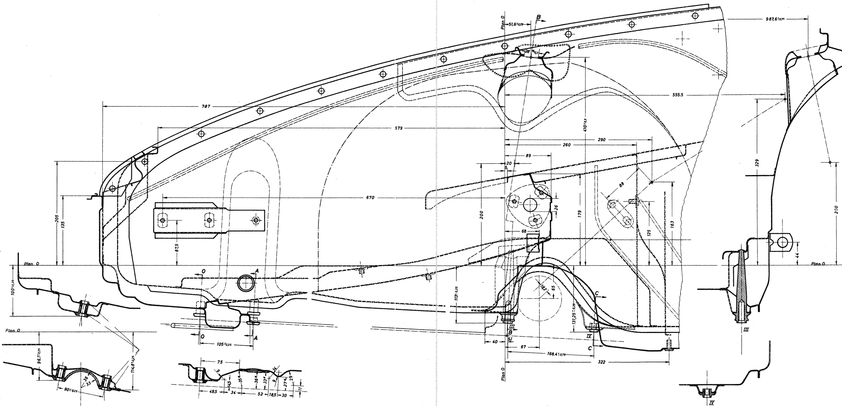
Check dimensions - front section
